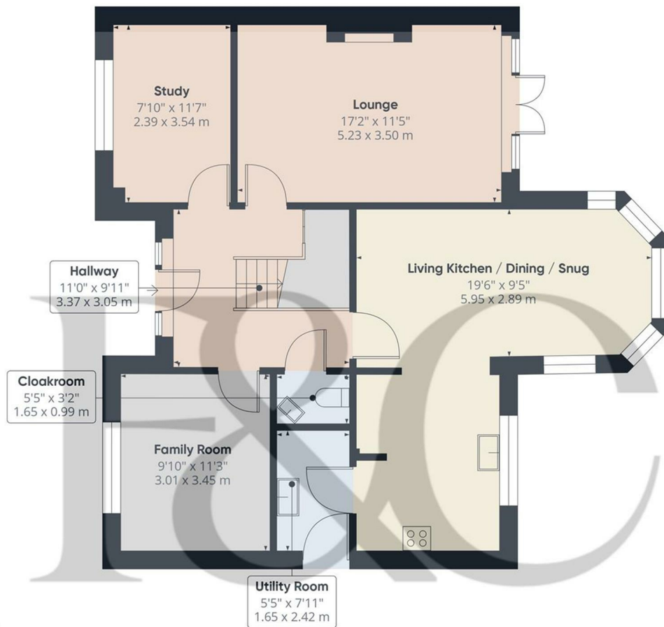
Floor 0 Building 1
