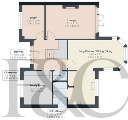
Floor 0 Building 1
